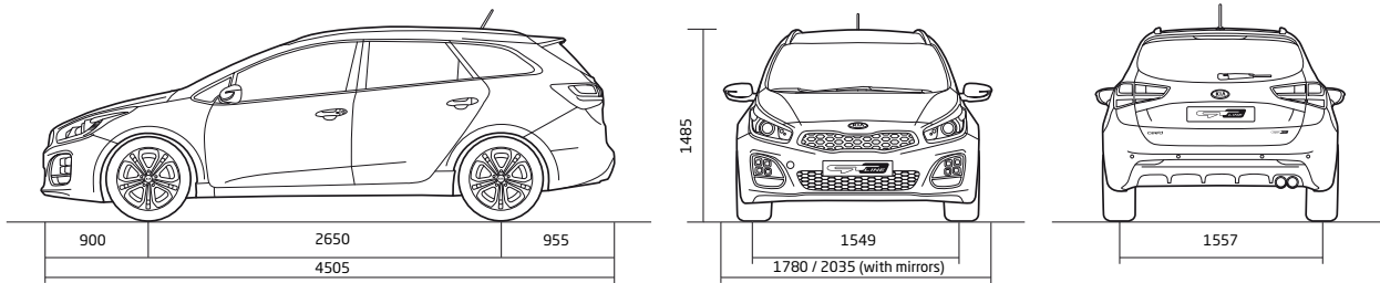
cee'd Sportswagon GT Line - yttre dimensioner (mm)
